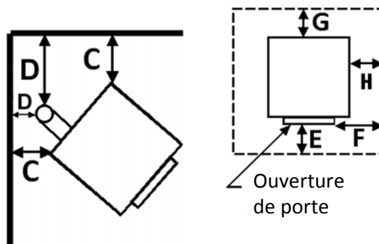
Figure 2 Installation en coin
