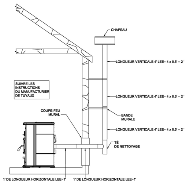
Figure 15 Évacuation murale
