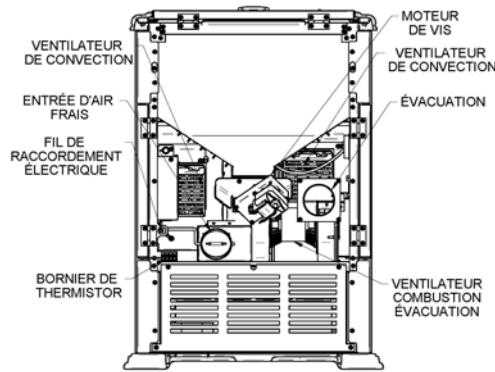
Figure 54 Composantes arrière
