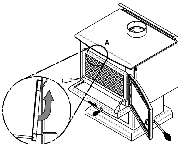
DETAIL A
